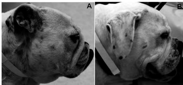
Figure 4. An example of a dog with a significant nose fold (A) covering the nose and a longer-muzzled dog without such fold (B). Photo source: Packer et al. 2015b
