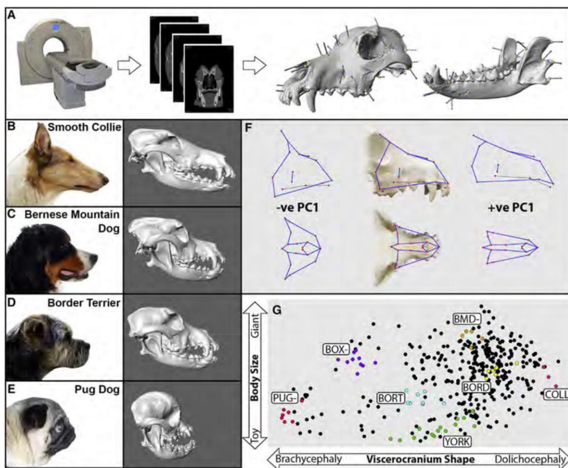
Fig. 2. Skull proportions with smooth-haired collie (B), Bernese mountain dog (C), border terrier (D) and mops (E). Photo source: Marchant et al. 2017.
